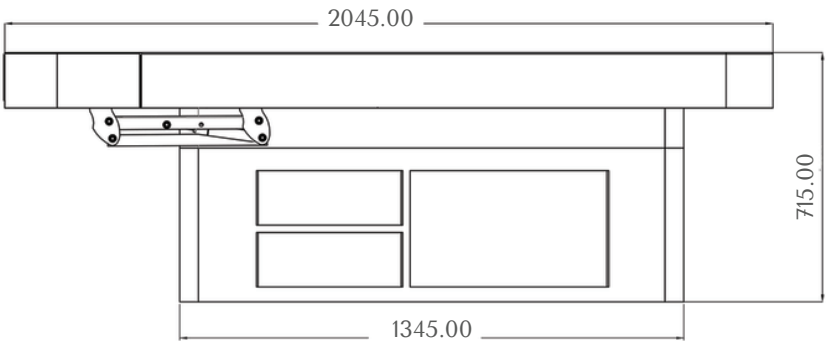
MINIMUM HEIGHT
