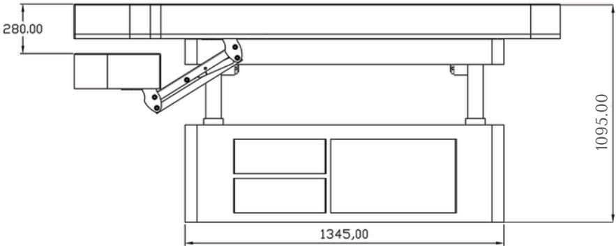
MAXIMUM HEIGHT
