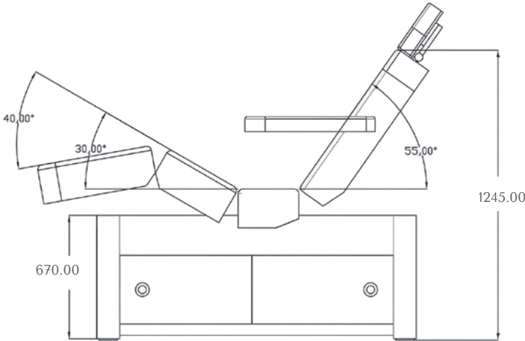
MINIMUM HEIGHT
