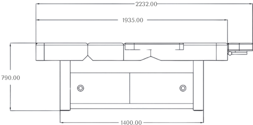
MAXIMUM HEIGHT
